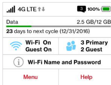
Data Usage
