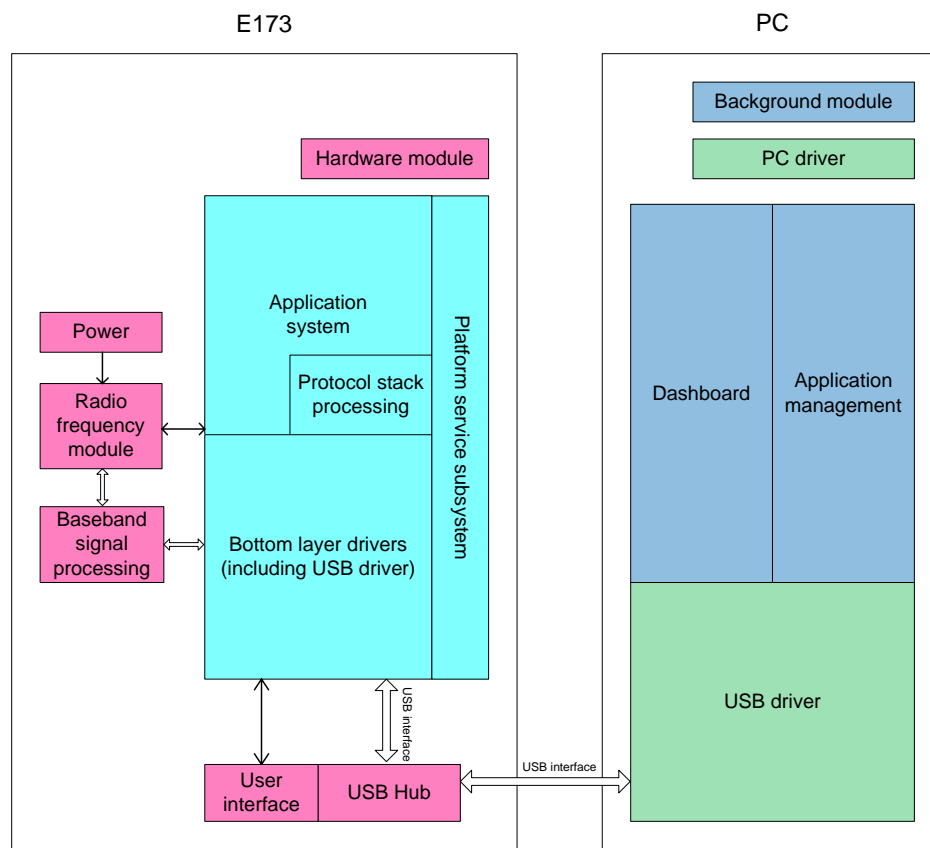
Figure 4-1 System architecture
