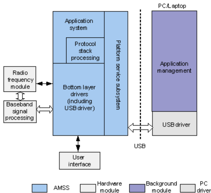
Figure 4-1 System architecture
