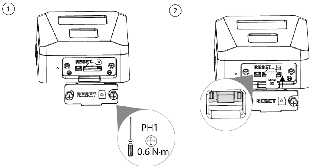
Figure 3-4 Install SD card
