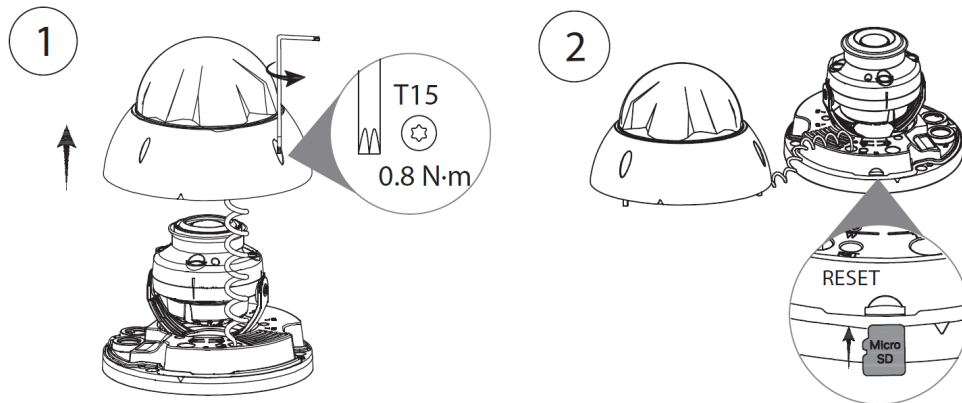
Figure 3-2 Install the SD card
