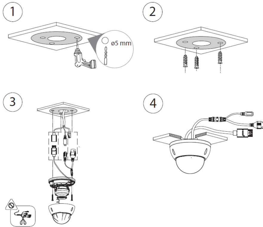
Figure 3-4 Cable going through the mounting surface
